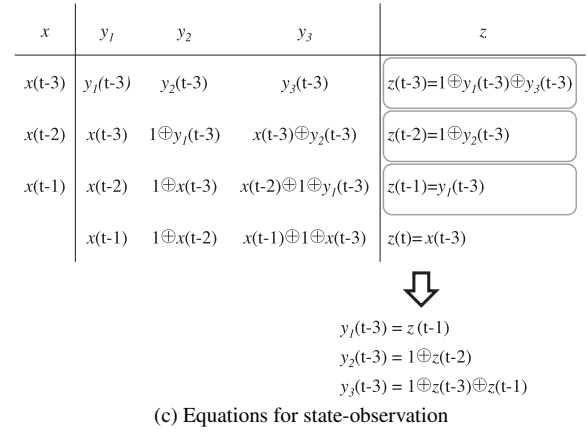
Fig. 6 State-justification and state-observation for R_2 .
