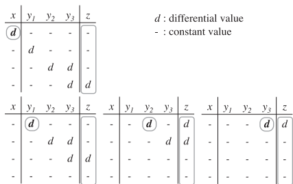
Fig. 12 Fundamental d-behaviors for S_1 .
