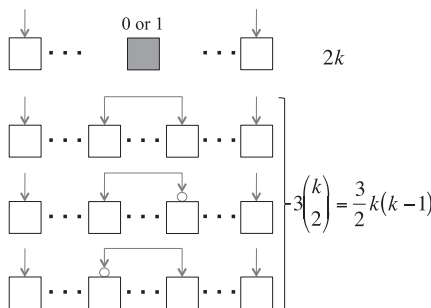
Fig. 14 Total number of patterns with one dummy FF.
