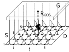
Figure 6: Scheme of the lumped MOS model
