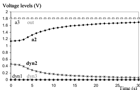
Figure 9: Influence of the GOS resistance
