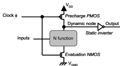
Figure 1: Domino logic gate (N type)
