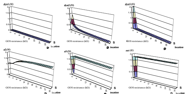
Figure 11: Influence of a 9-node GOS in Na on voltage levels
