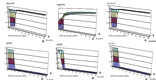
Figure 12: Influence of a 9-node GOS in Ppr on voltage levels
