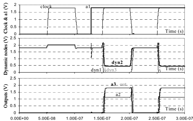
Figure 8: Time diagrams of the voltage levels, GOS in Na (1 node centered, 1\Omega , 10MHz)
