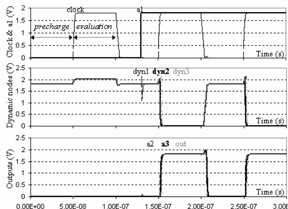
Figure 3: Timing diagrams of the healthy Domino structure at 10MHz
