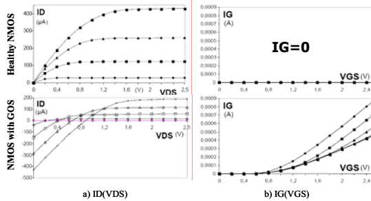
Figure 5: Typical characteristics of Drain (a) and Gate (b) currents for a healthy NMOS (top) and a NMOS affected by a GOS (bottom)
