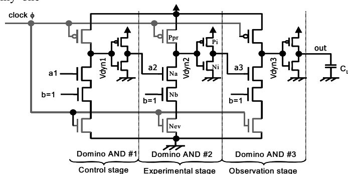
Figure 2: Domino logic structure of study (chain of 3 AND cells)
