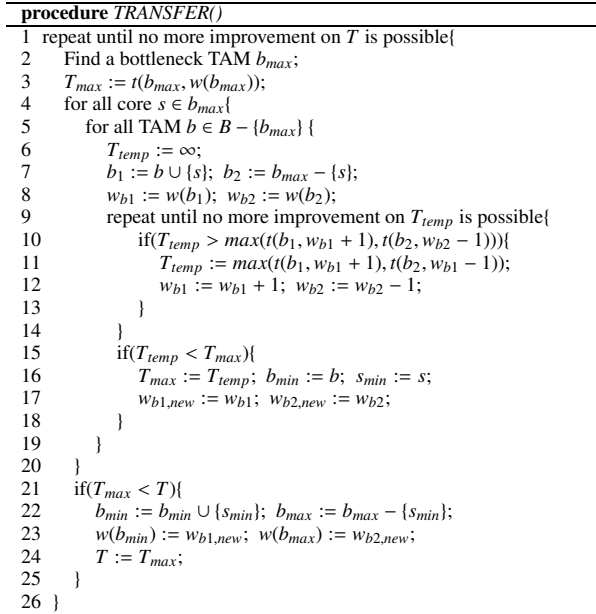
Figure 7. TRANSFER procedure
