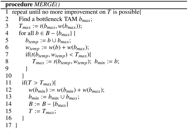
Figure 9. MERGE procedure
